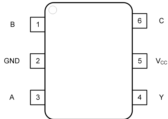
Fig. 2. Top view pin configuration SOT23-6 and SOT363
