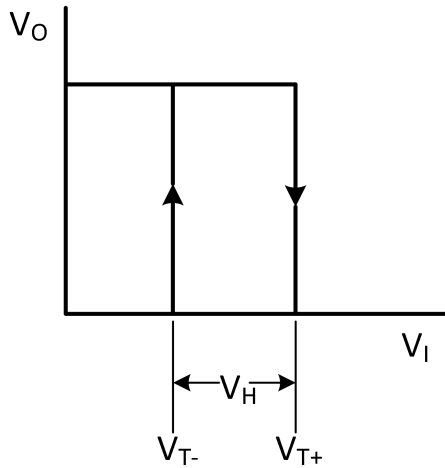
Fig. 12. Transfer characteristic
