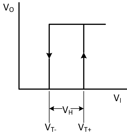
Fig. 14. Transfer characteristic
