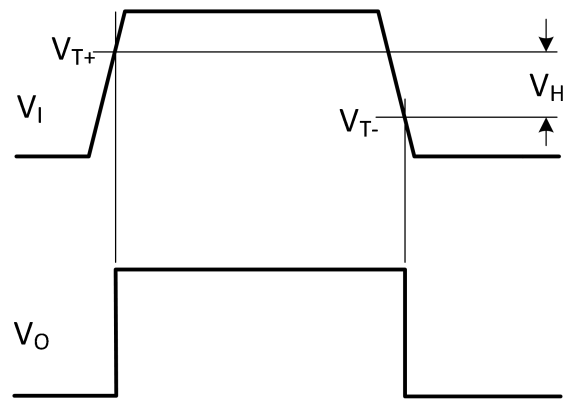
Fig. 13. Definition of V_{T+} , V_{T-} and V_H
