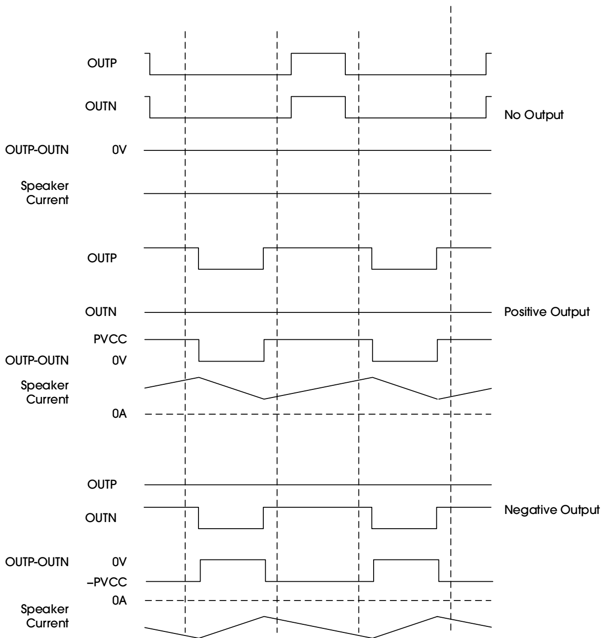
Figure 7. Low-Idle-Current 1SPW Modulation
