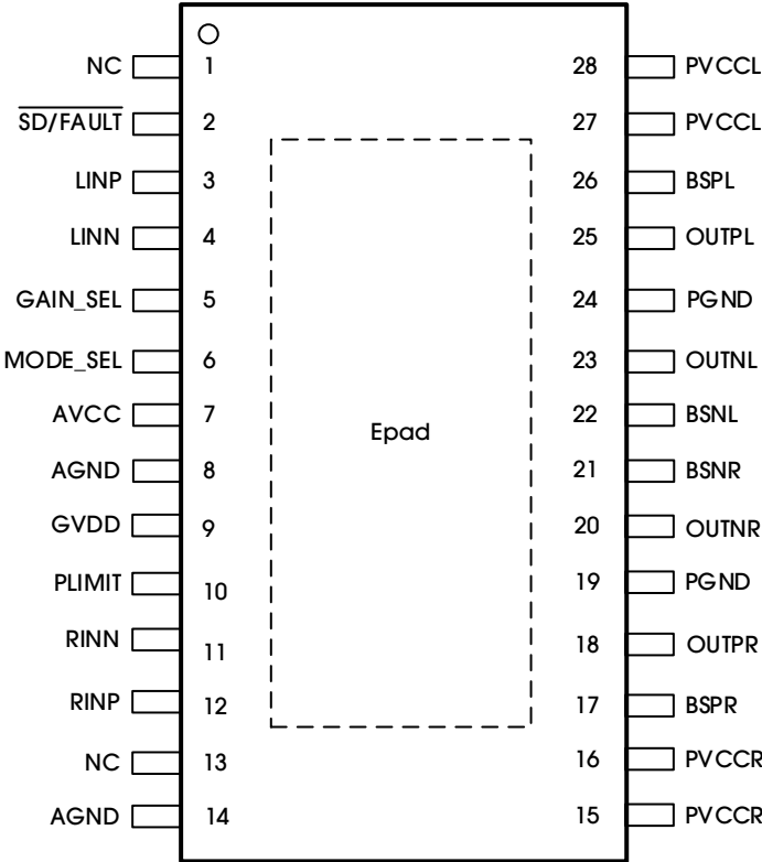
Figure 1. Pin Configuration
