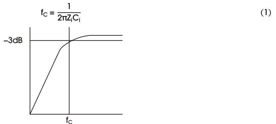
Figure 13. Input Filter
