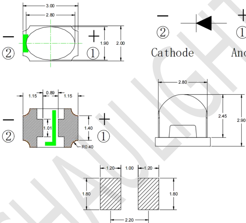
推荐焊盘尺寸 Recommend Pad size
