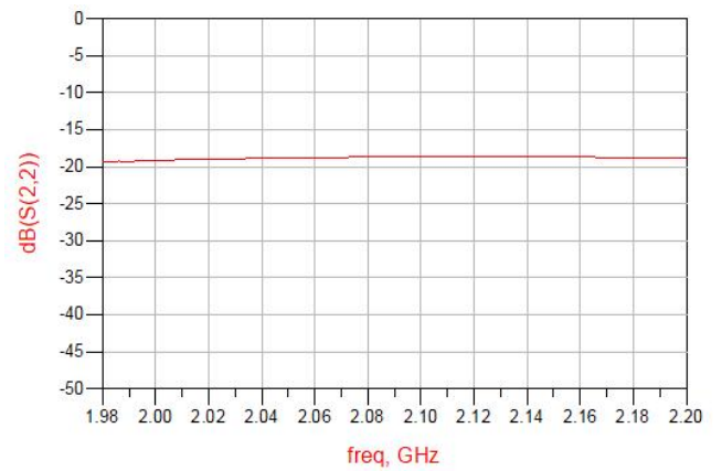
Figure 8. MQF2108G1 Return Loss (S22)
