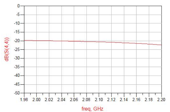
Figure 10. MQF2108G1 Return Loss (S44)
