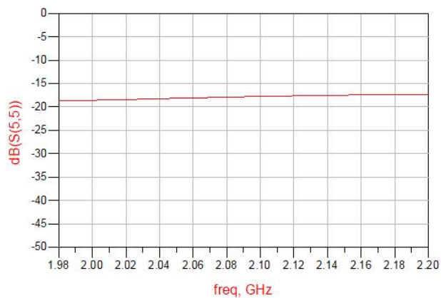
Figure 11. MQF2108G1 Return Loss (S55)
