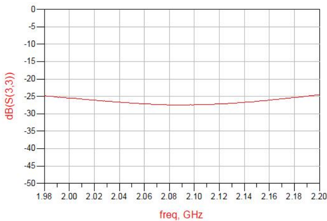
Figure 9. MQF2108G1 Return Loss (S33)
