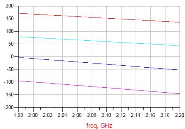
Figure 12. MQF2108G1 Phase
