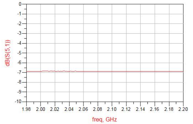
Figure 6. MQF2108G1 Coupling
