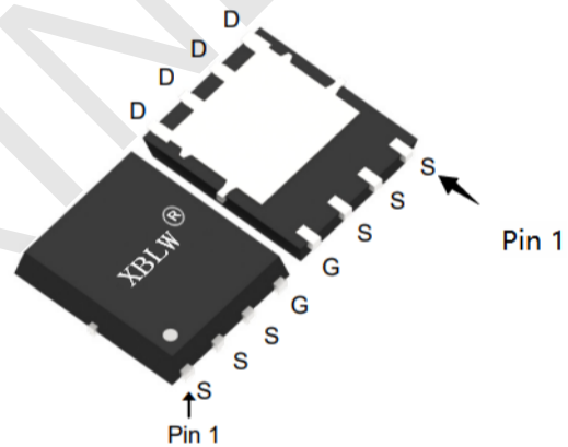
DFN5X6-8L
