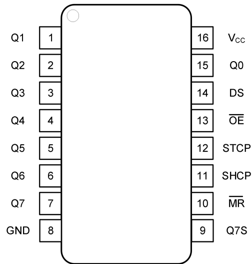
Fig. 5. Top view pin configuration SOP, SSOP and TSSOP
