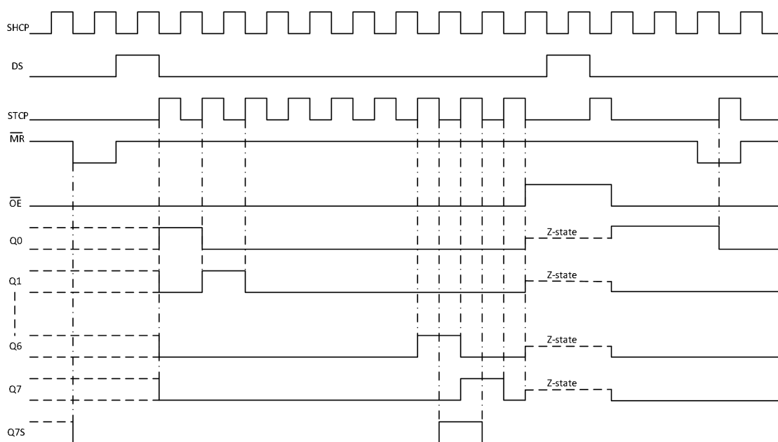
Fig. 6. Timing diagram
