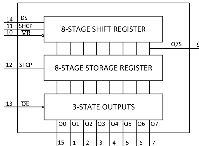
Fig. 1. Functional diagram
