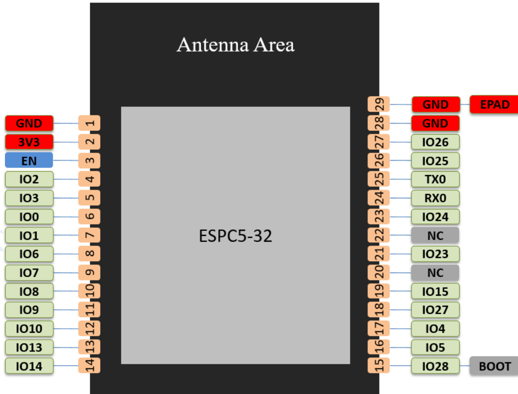
Fig.2.1 ESPC5-32 Pins Definition (Top view)
