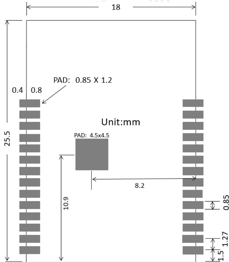
Fig. 3.3 PCB Layout for ESPC5-32 (Top view)
