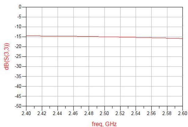
Figure 9. MQF2508G1 Return Loss (S33)
