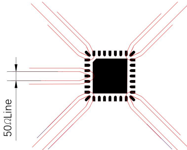
Figure 13. Recommended PCB Layout
