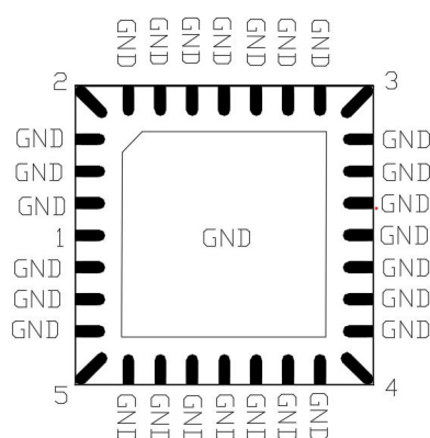
Figure 1. MQF2508G1 (Bottom View)
