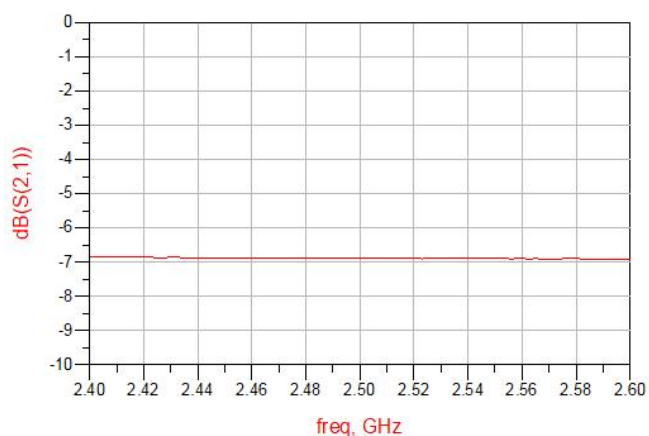
Figure 3. MQF2508G1 Coupling
