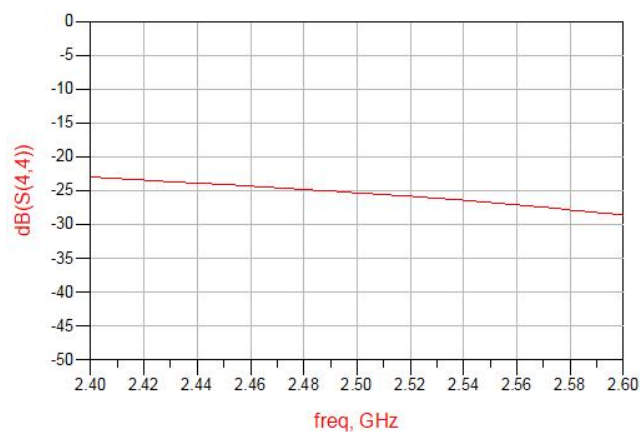
Figure 10. MQF2508G1 Return Loss (S44)
