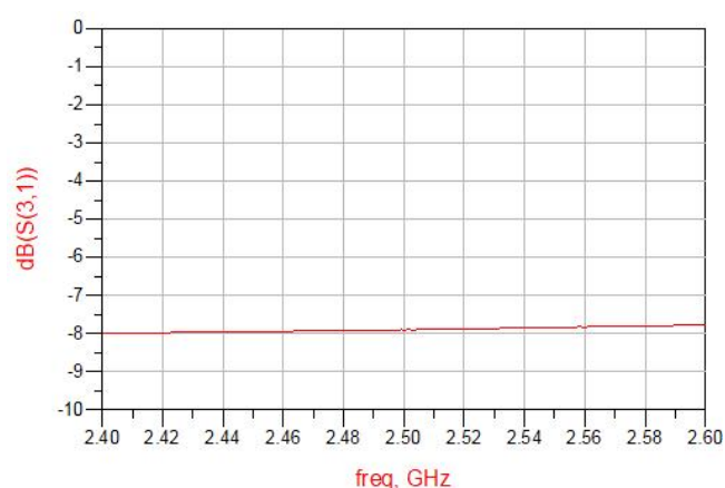
Figure 4. MQF2508G1 Coupling
