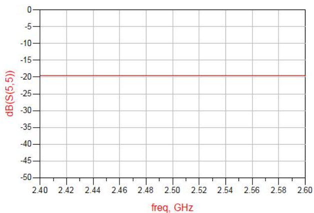
Figure 11. MQF2508G1 Return Loss (S55)
