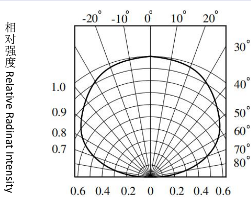
Relative Radiant Intensity vs. Angular Displacement
