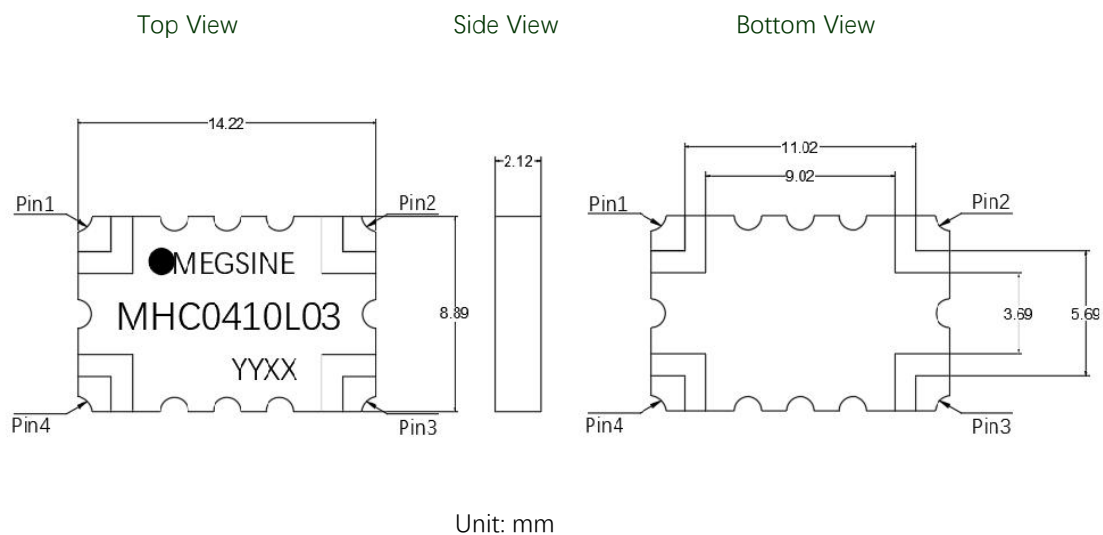
Figure 2. MHC0410L03 Outline Drawing
