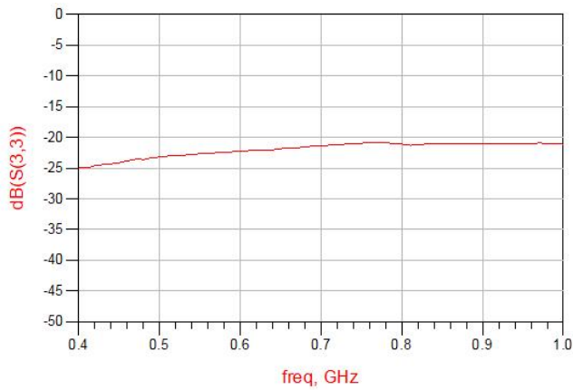
Figure 7. MHC0410L03 Return Loss (S33)
