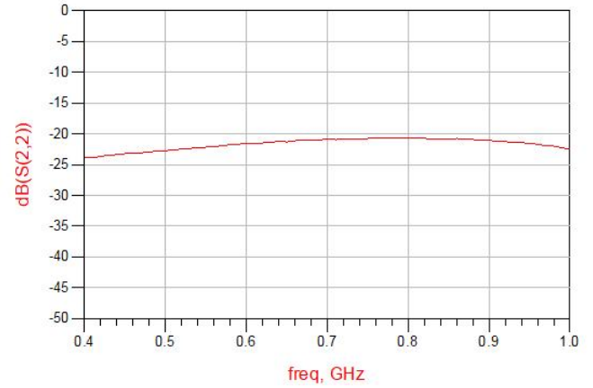
Figure 6. MHC0410L03 Return Loss (S22)
