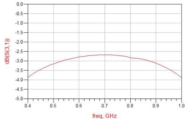
Figure 4. MHC0410L03 Transmission
