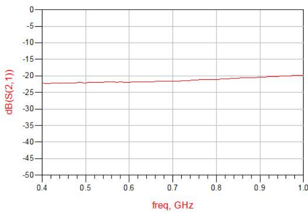
Figure 9. MHC0410L03 Isolation
