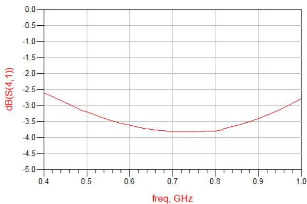
Figure 3. MHC0410L03 Coupling
