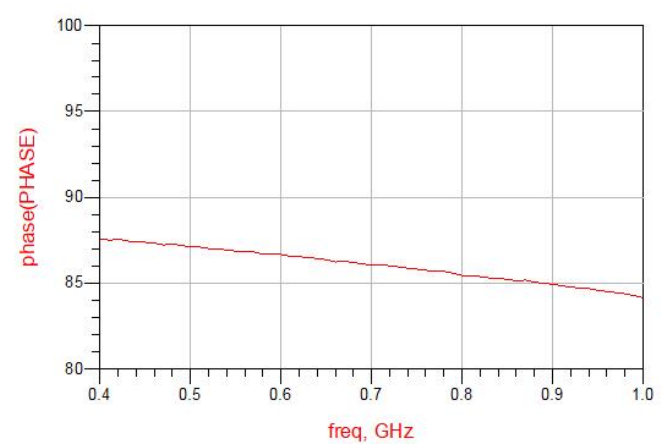
Figure 10. MHC0410L03 Phase
