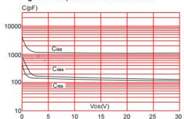
Figure 6: Capacitance Characteristics
