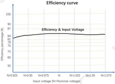
Figure 6: Efficiency VS Input Voltage (100% Load)
