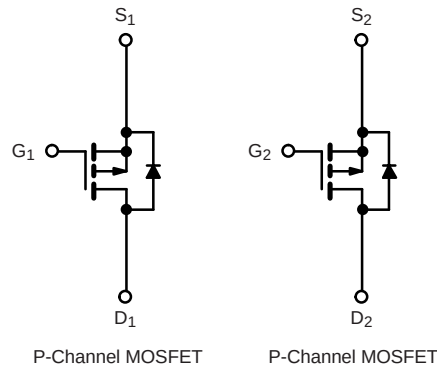
PowerPAK SC-70-6 Dual
