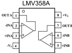
SOP-8/MSOP-8/DIP-8/TSSOP-8
