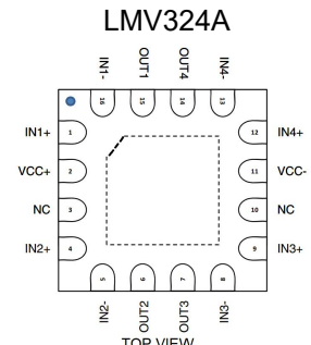
QFN-16 3*3
