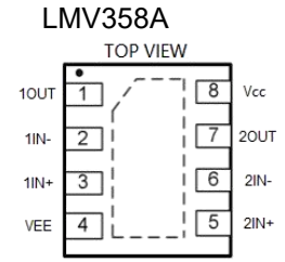
DFN-8 2*2/DFN-8 3*3
