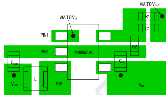
Figure 3. M8088AAC Suggested Layout
