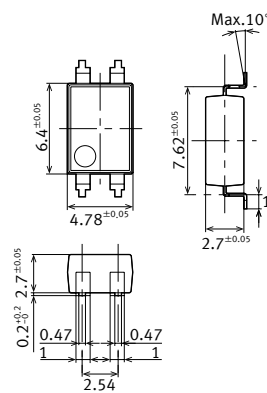
Surface mount terminal type
