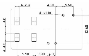
KT206-L/D MA 单线圈 Single coil
