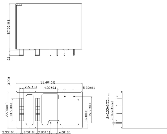
KT206-L/D 单线圈 Single coil
