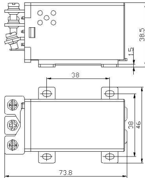
T：铁板安装型:Iron plate mounting type
