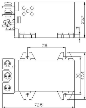
塑壳安装型 Molded case mounting type
