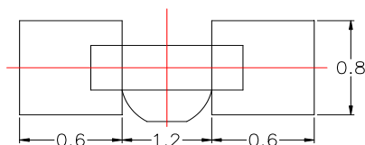
Recommended Soldering Pad Dimensions
