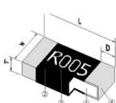
四位数白色标记 Four digit white marking (1206 > R001, 2010, 2512, 2817, 4527)
