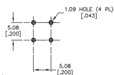
P.C. MOUNTING
