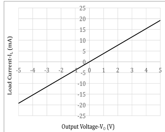
Fig.2 Current vs. Voltage Characteristics Of Output At MOS Portion
