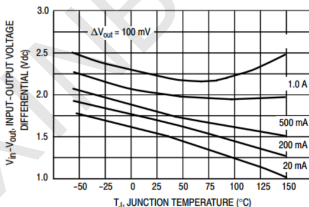
Dropout Voltage
