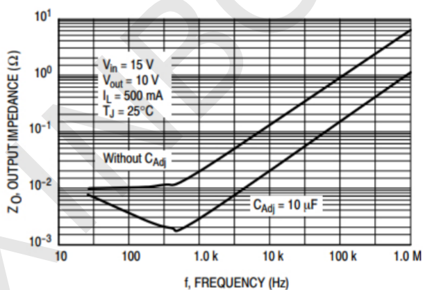
Output Impedance
