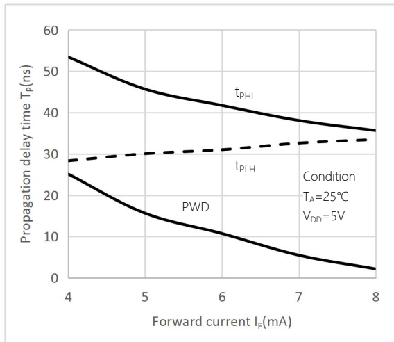
Fig.5 Propagation delay time vs. Forward current
