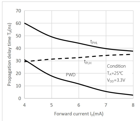
Fig.6 Propagation delay time vs. Forward current
