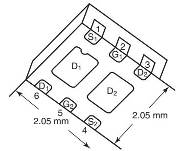
PowerPAK SC-70-6 Dual
