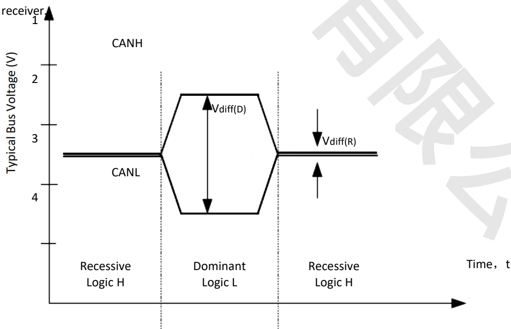
Bus States (Physical Bit Representation)
