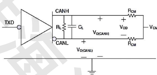
Driver Test Circuit and Measurement
