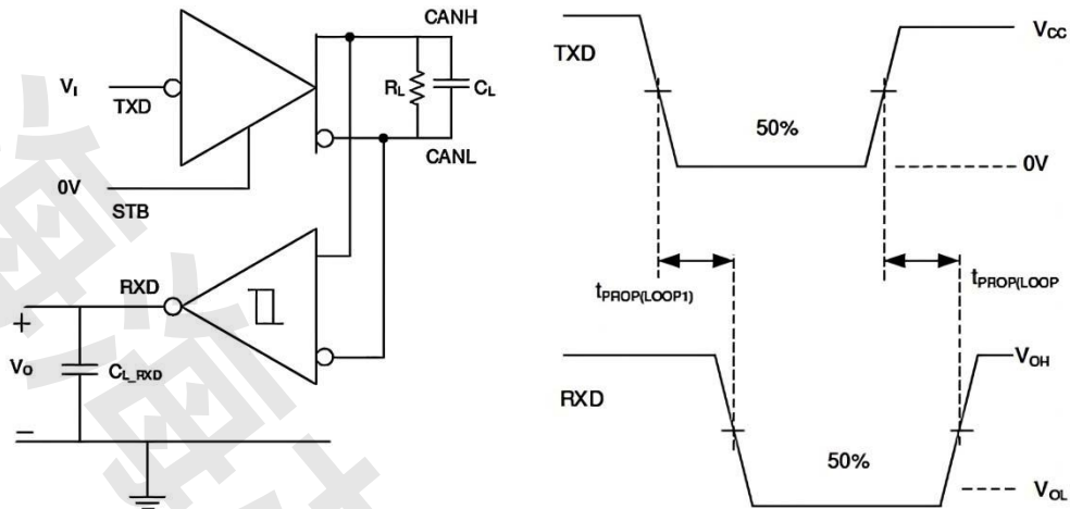
T_{PROP(LOOP)} Test Circuit and Measurement
