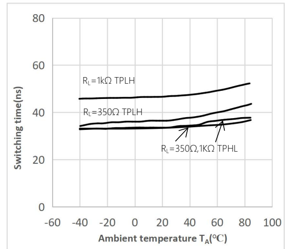
Fig.8 Switching time vs. Ambient temperature
