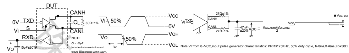
F7. tEN Test Circuit and Voltage Waveforms
