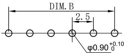
PCB LAYOUT
