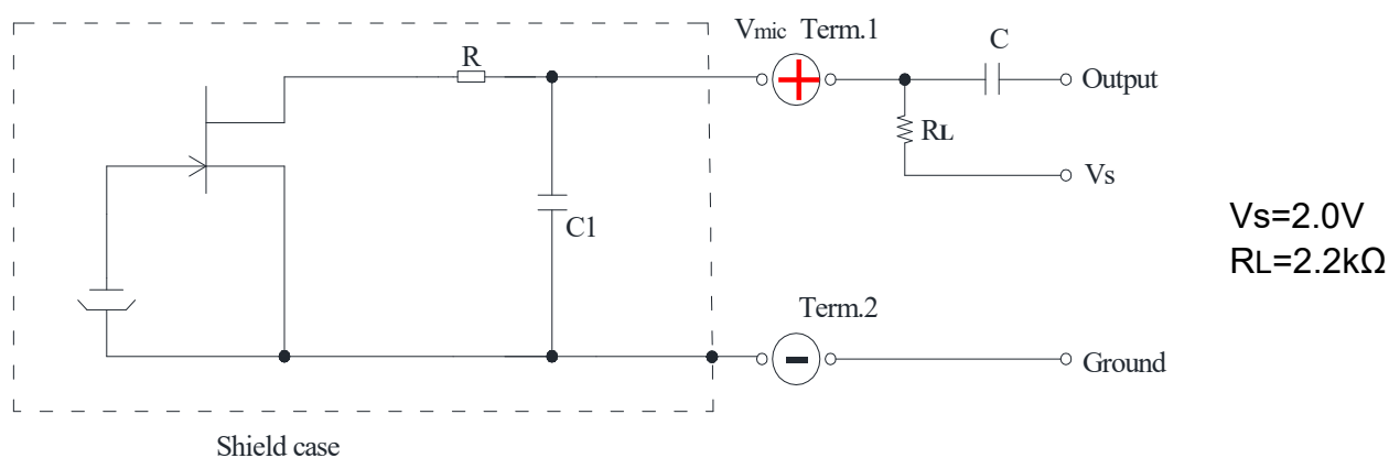
Fig. 5-1 Schematic Diagram
