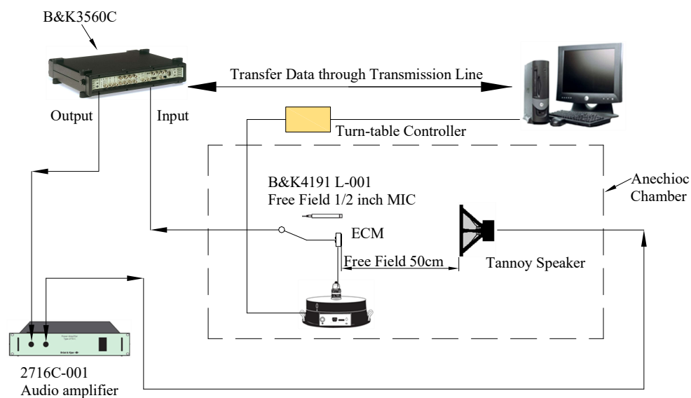
Fig. 6-1 Measurement System Setup
