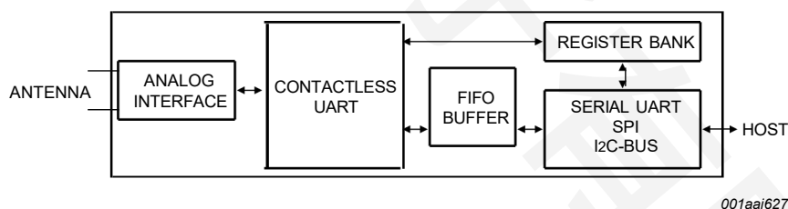
Fig 1. Simplified block diagram of the MFRC522
