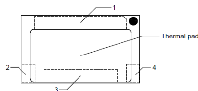
Package Outline
