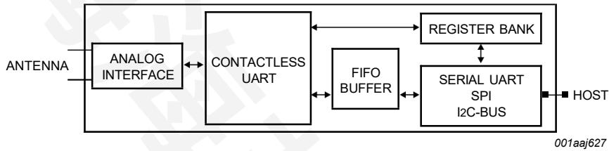
Fig 1. Simplified block diagram of the MFRC523
