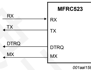
Fig 8. UART connection to microcontrollers
