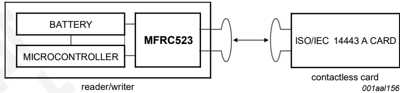
Fig 4. MFRC523Read/Write mode
