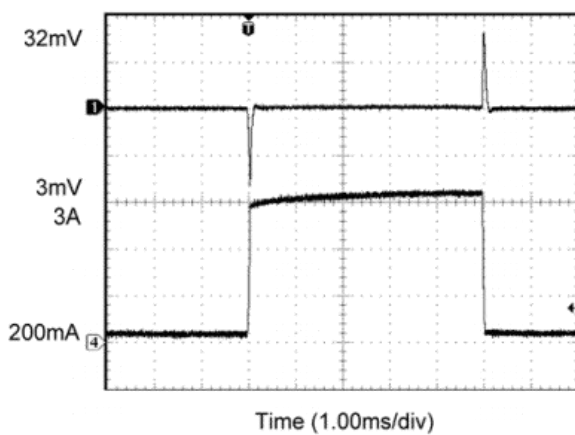
MIC29302 Load Transient Response
