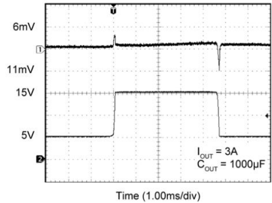
MIC29302 Line Transient Response with 3A Load, 1000μF Output Capacitance
