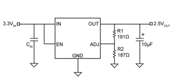
MIC29302 Adjustable Output Regulator
