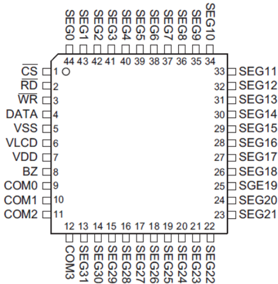
HT1621B 44LQFP-A
