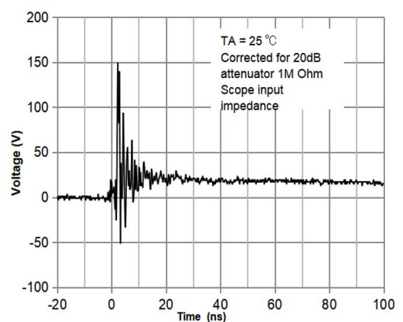
TLP Measurement
