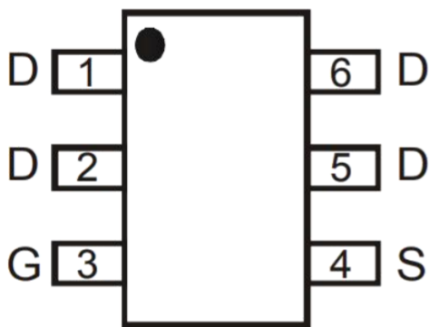
Top View SOT363
