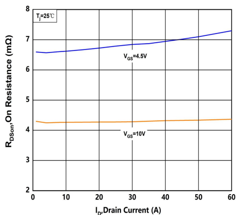
Figure.3 On-Resistance vs Drain Current For Various Gate Voltage
