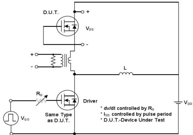
Peak Diode Recovery dv/dt Test Circuit
