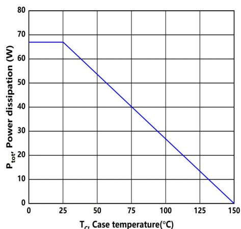
Figure.10 Maximum power Dissipation Derating vs Case Temperature
