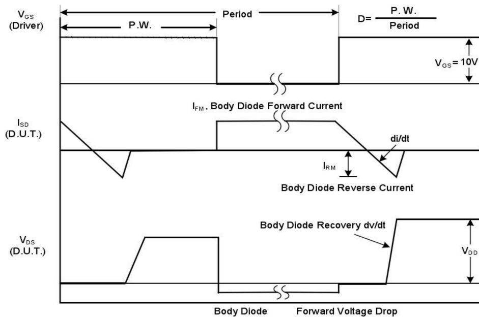
Peak Diode Recovery dv/dt Waveforms
