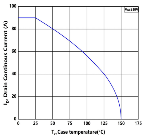
Figure.11 Continuous Drain Current Derating vs Case Temperature
