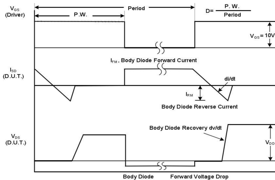
Peak Diode Recovery dv/dt Waveforms
