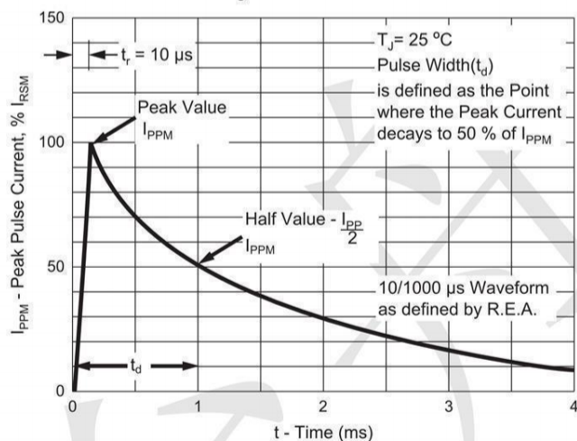
Fig. 3 - Pulse Waveform
