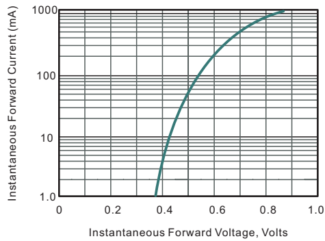
Fig.4 Typical Forward Voltage
