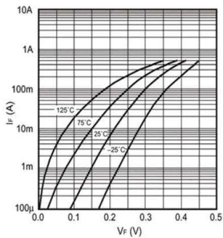
Fig.1 Forward characteristics
