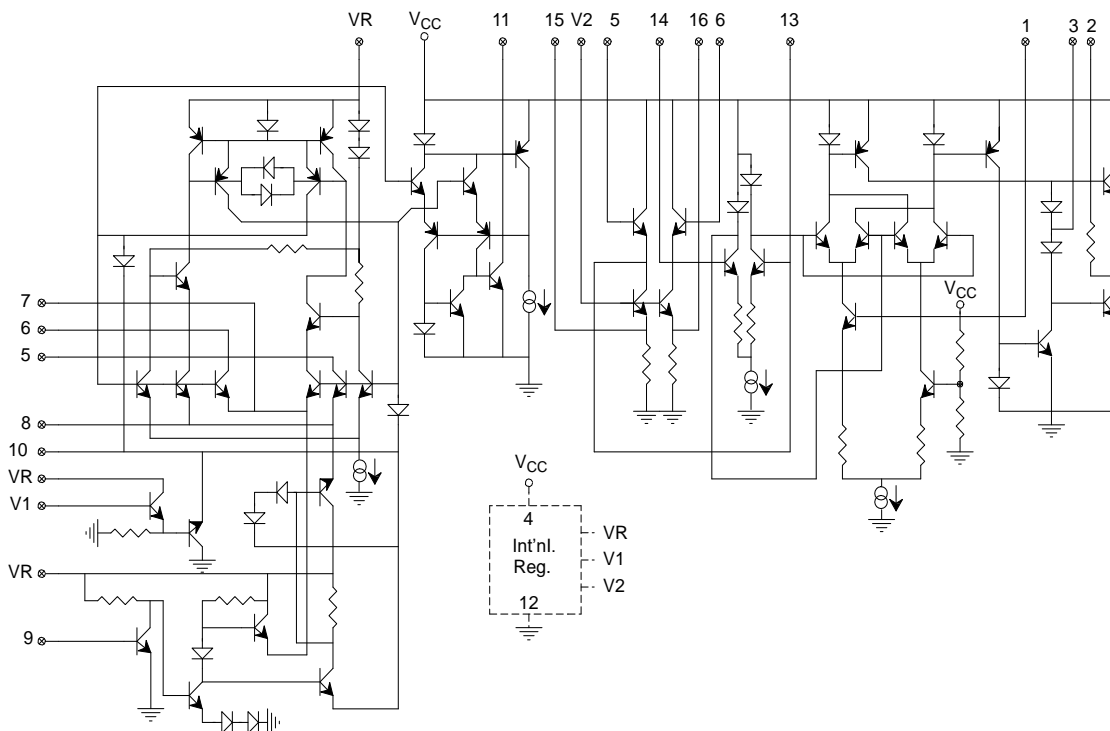
Figure 15. Equivalent Schematic Diagram
