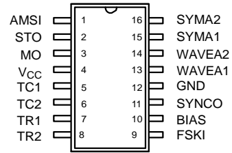
16 Lead SOP
