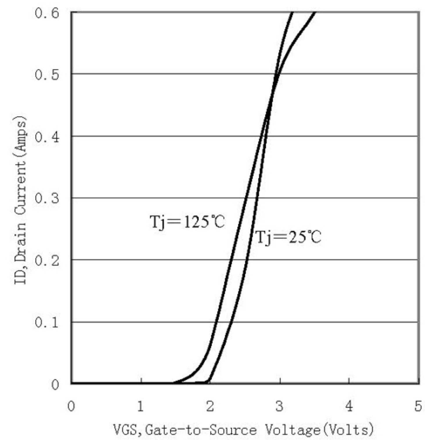
Figure 2. Transfer Characteristics
