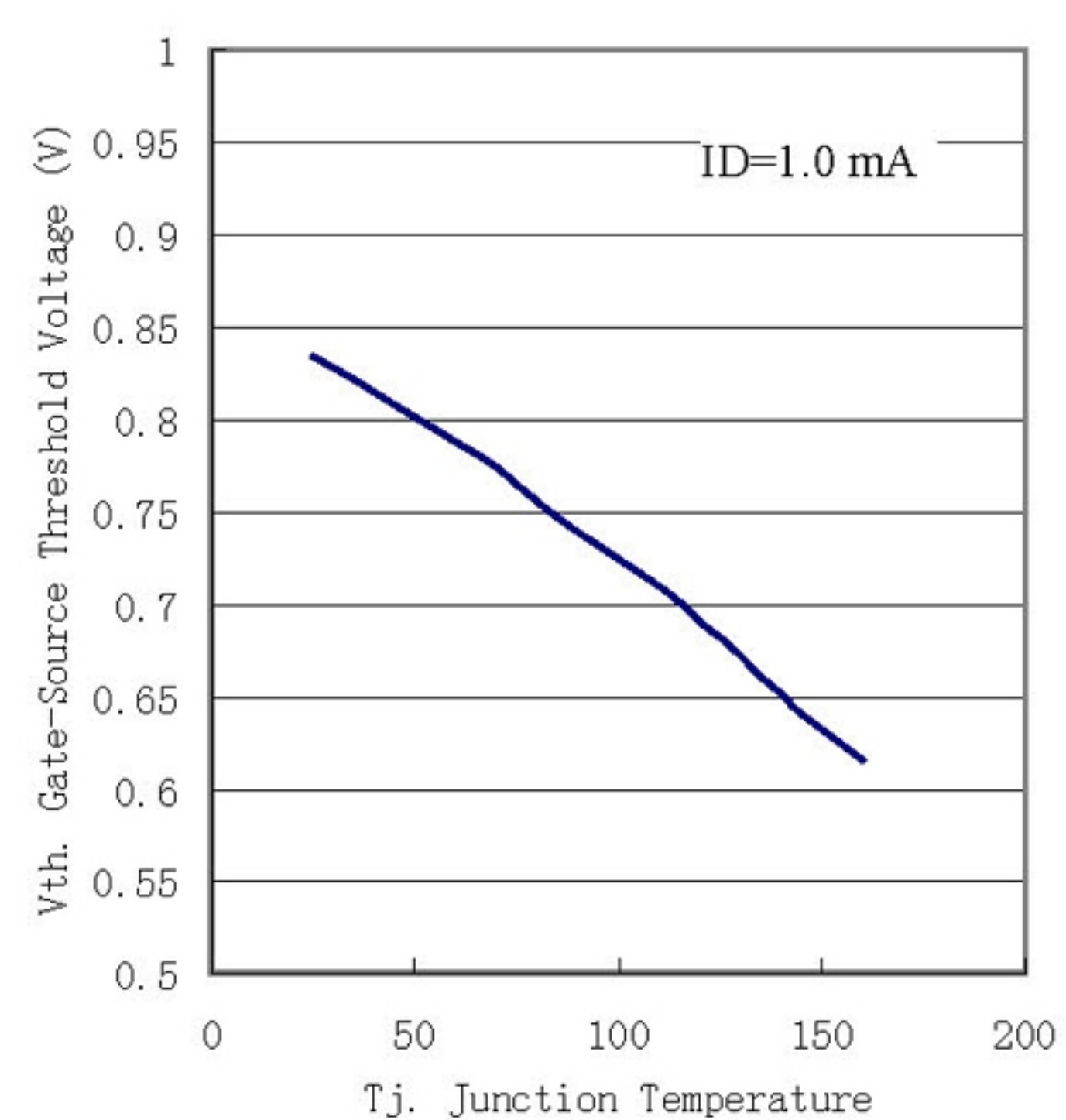
Figure 4. Gate Threshold Variation with Temperature
