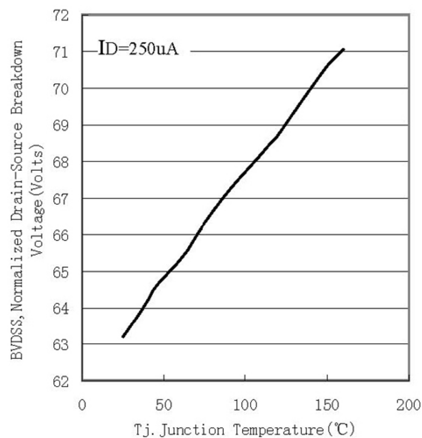
Figure 3. Breakdown Voltage Variation with Temperature
