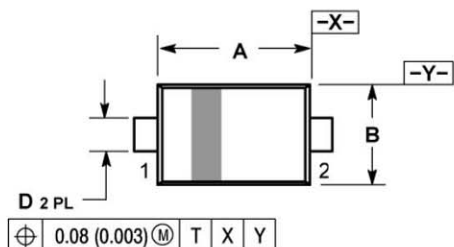
SOD-523 CASE 502-01 ISSUE A
