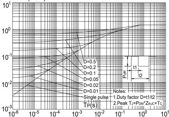
Figure.11: Maximum Effective Transient Thermal Impedance, Junction-to-Case Z_{thj-c}(^{\circ}C/W)
