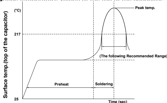
TEMPERATURE PROFILE
