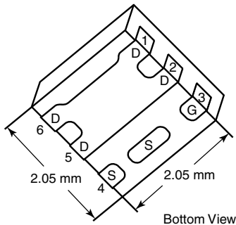
DFN2X2
