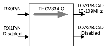
1Lane V-by-One® HSII In / Single-Link oLDI Out
