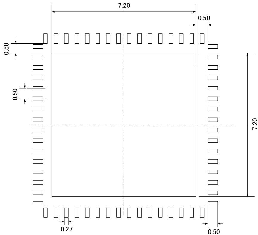
TOP VIEW
