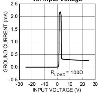
2950x Ground Current vs. Input Voltage
