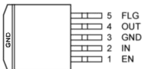
5-Pin TO-263 Fixed Voltage LM29151/29301/29501
