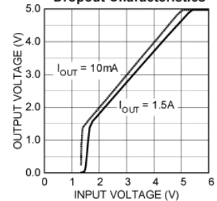
29150-5.0 Dropout Characteristics
