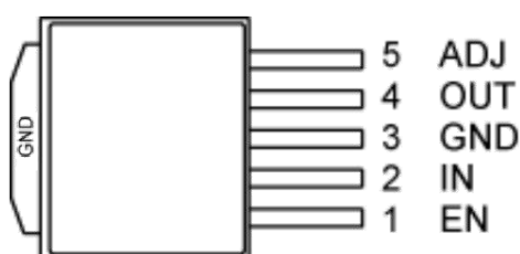
5-Pin TO-252 Adjustable Voltage LM29152
