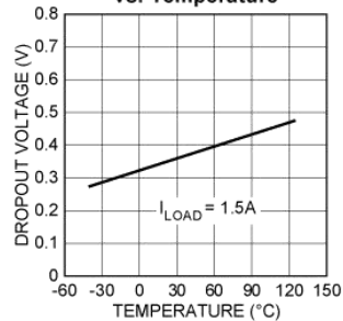
2915x Dropout Voltage vs. Temperature
