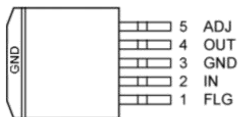
5-Pin TO-263 Adjustable with Flag LM29153/29303/29503
