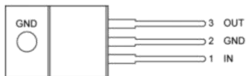
3-Pin TO-220 LM29150/29300/29500
