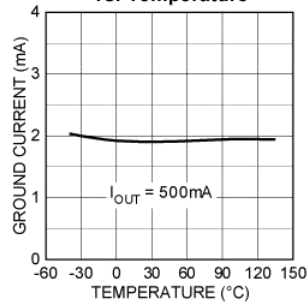
2950x Ground Current vs. Temperature
