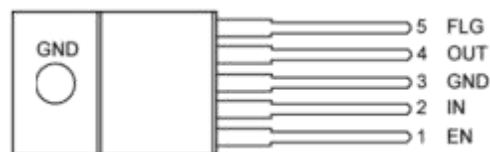
5-Pin TO-220 Fixed Voltage LM29151/29301/29501/29751
