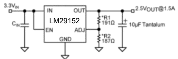
Adjustable Output Voltage (*See Minimum Load Current Section)
