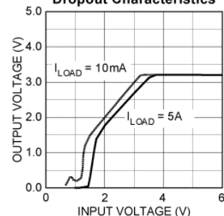
29500-3.3 Dropout Characteristics
