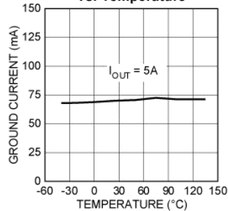
2950x Ground Current vs. Temperature
