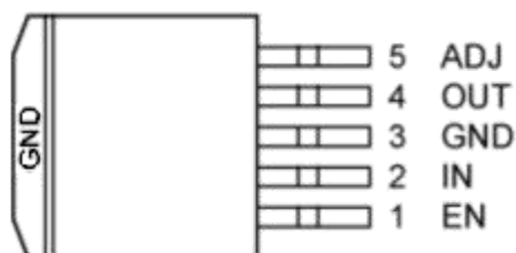
5-Pin TO-263 Adjustable Voltage LM29302A/29502
