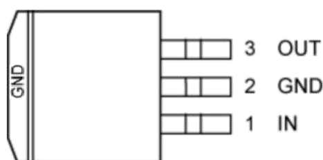
3-Pin TO-263 LM29150/29300
