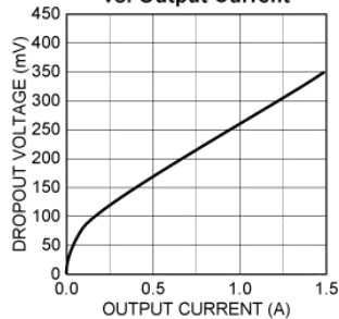
2915x Dropout Voltage vs. Output Current
