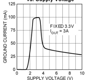
2930x Ground Current vs. Supply Voltage
