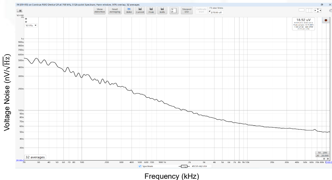
Input Voltage Noise Spectral Density vs. Frequency
