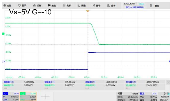
Overload Recovery Time
